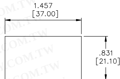
Panel Cutout
