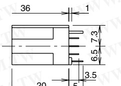
PC Board Terminal with Built-in Resistor (AL-C2□V)
