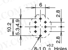
Panel Cut-out Bottom View
