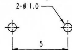
P.C.B MOUNTING DIMENSIONS
