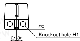
Fig. 2 Plastic enclosure
