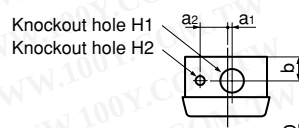
Fig. 1 Plastic enclosure
