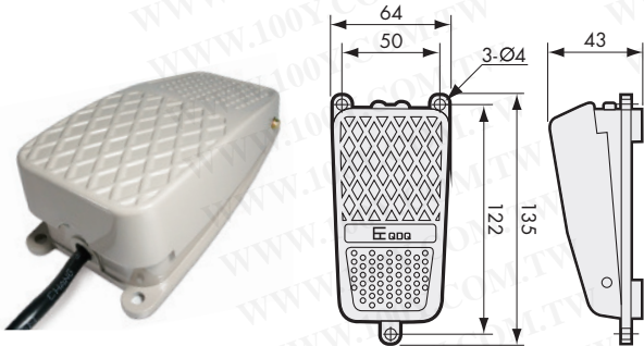
CT-H3N 15A 250VAC, 金屬Metal 動作壓力Operating pressure: 3.2kg
