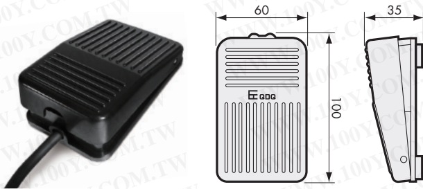
CT-M1 10A 250VAC, 塑膠Plastic 動作壓力Operating pressure: 0.7kg
