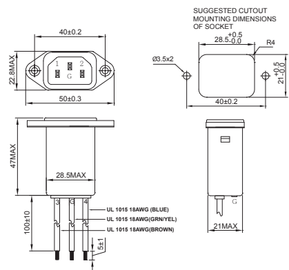
YB-A (lead-wire)
