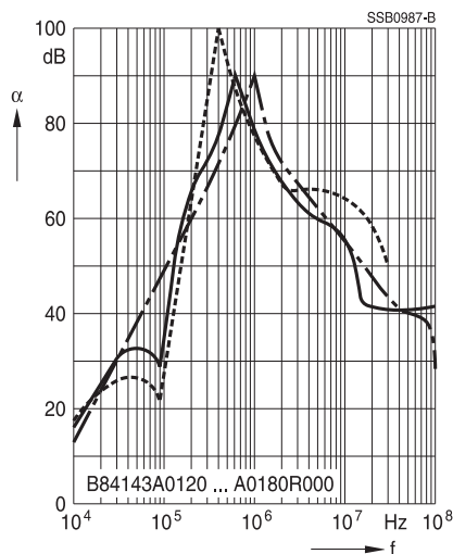
Filters for 120 A ... 180 A
