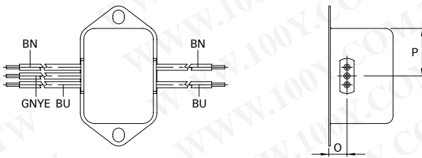
Connection style -08, 20A types
