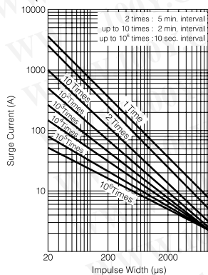
Impulse Derating (Relation between impulse width and impulse repetition times) (ERZV10D820 to ERZV10D511)
