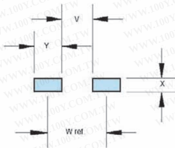
Land Pattern
