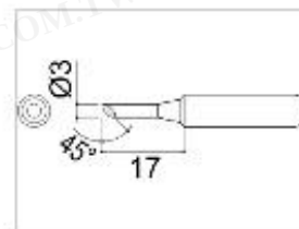
900M-T-3CF Shape-3C Tinned cut surface only
