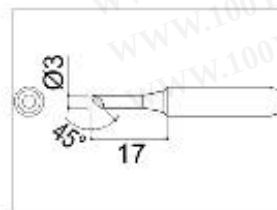
900M-T-3C Shape-3C
