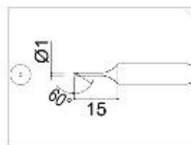
900M-T-1CF Shape-1C Tinned cut surface only
