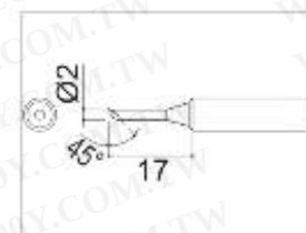
900M-T-2CF Shape-2C Tinned cut surface only
