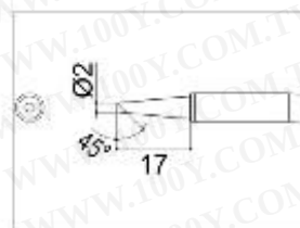
900M-T-2BCZ Shape-2BC (Z) * Long Life Type
