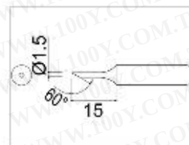
900M-T-1.5CF Shape-1.5C Tinned cut surface only
