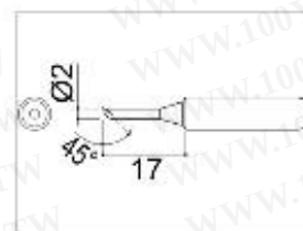
900M-T-2C Shape-2C
