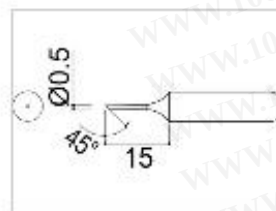
900M-T-0.5C Shape-0.5C
