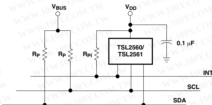
Figure 15. Bus Pull-Up Resistors
