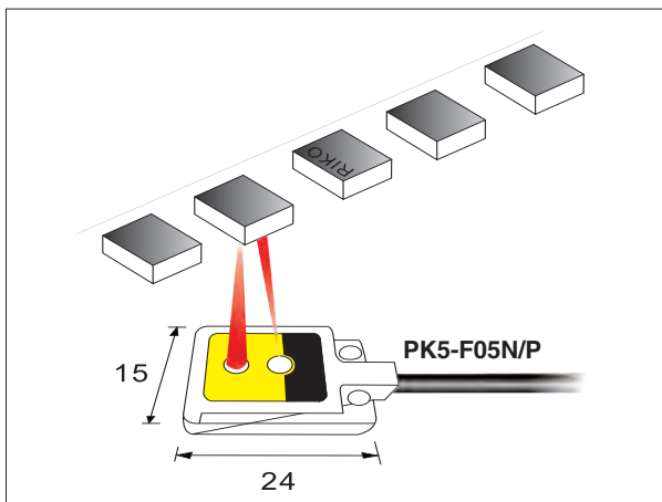
檢測PCB定位 Detecting presence of object.
