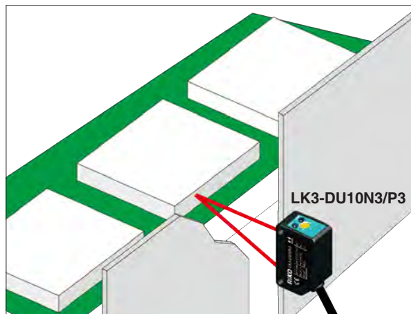
零件檢測 Detecting parts.
