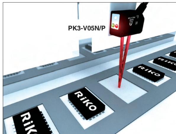
檢測有無IC Detecting if the IC is existed or not.
