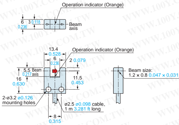
PM-U25 Sensor
