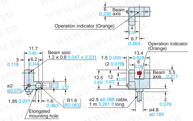
PM-F25 Sensor
