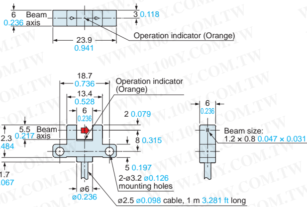
PM-K25 Sensor
