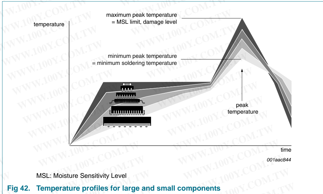
Fig 42. Temperature profiles for large and small components For further information on temperature profiles, refer to Application Note AN10365 “Surface mount reflow soldering description”.
