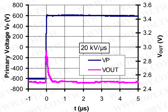
Figure 18: dv/dt
