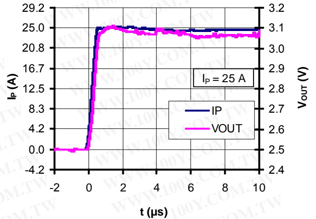
Figure 16: Step response
