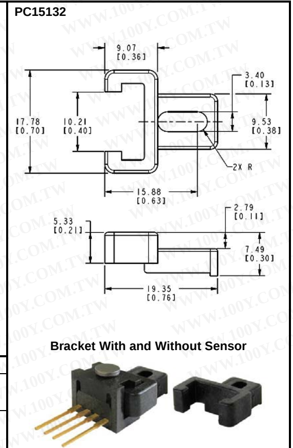
Figure 3. Plastic Mounting Bracket Mounting Dimensions (For reference only: mm/[in.] )
