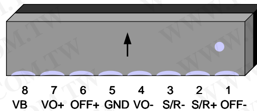
HMC1051ZL Pinout
