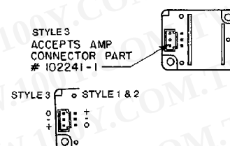
PINOUT STYLES
