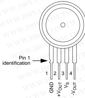
Figure 2. Device pinout (front view)
