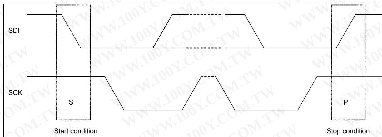
Figure 12: Timing diagram for I 2 C start and stop condition (SDI=SDA)
