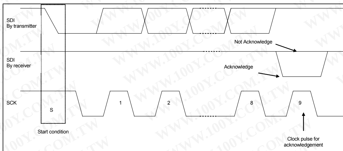
Figure 14: Timing diagram for I 2 C acknowledgement on SDI (SDI=SDA)
