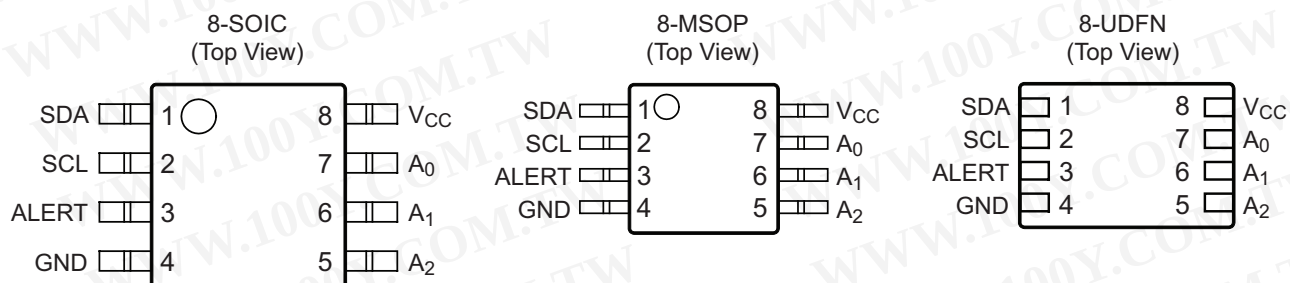
Figure 1. Pin Configurations
