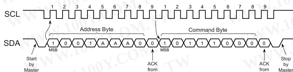
Figure 9-2. Copy Nonvolatile Registers to Volatile Registers
