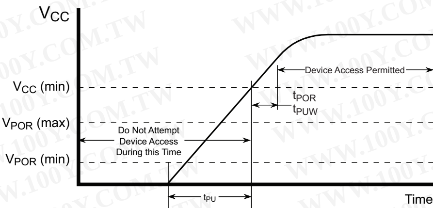
Figure 11-2. Power-up Timing
