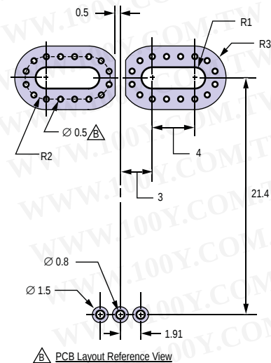
PCB Layout Reference View
