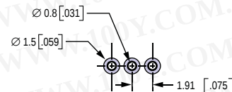
Recommended PCB Layout View
