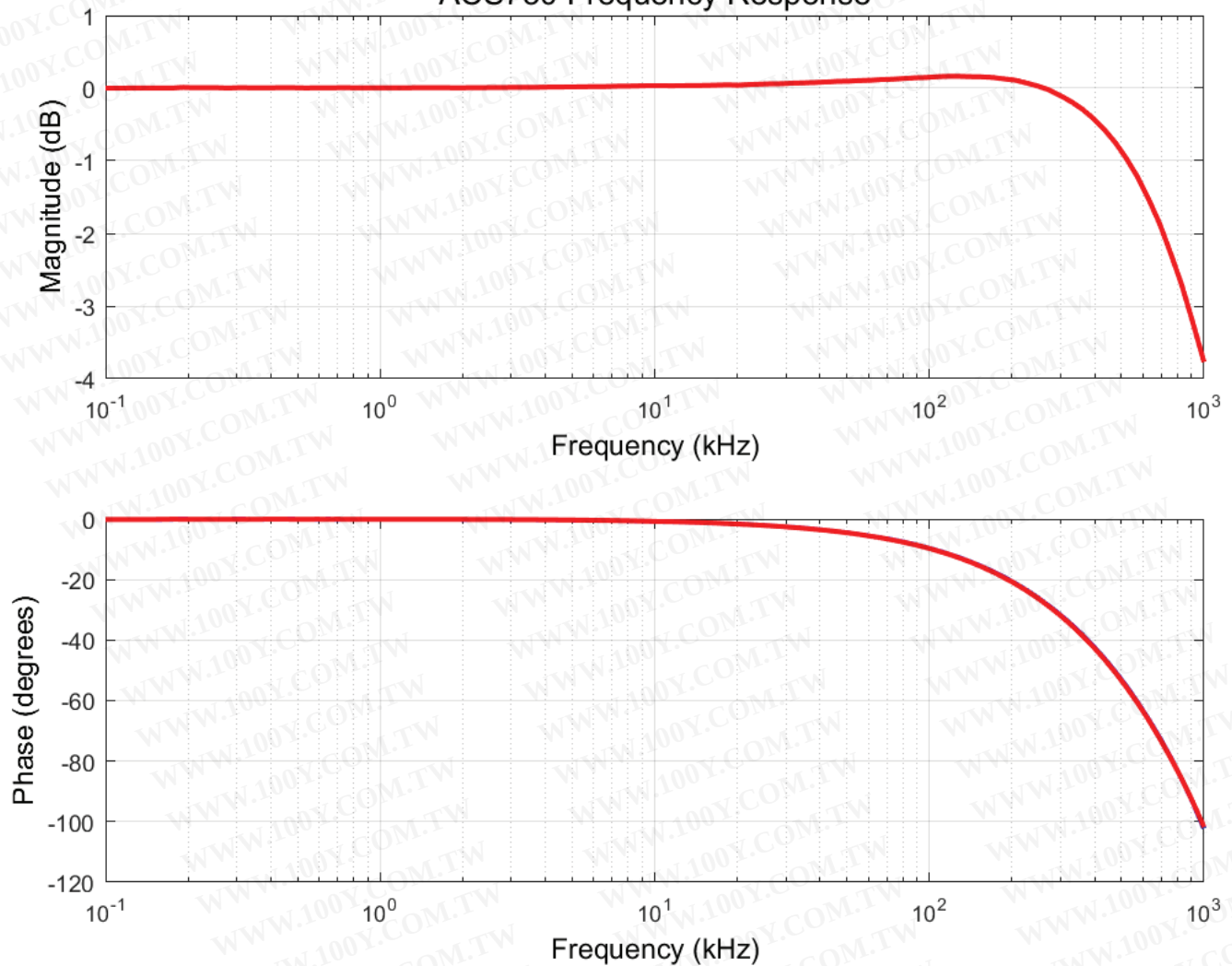
ACS730 Frequency Response
