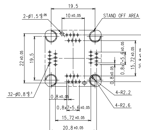
P.C.B PATTERN (2:1) (TOP VIEW)
