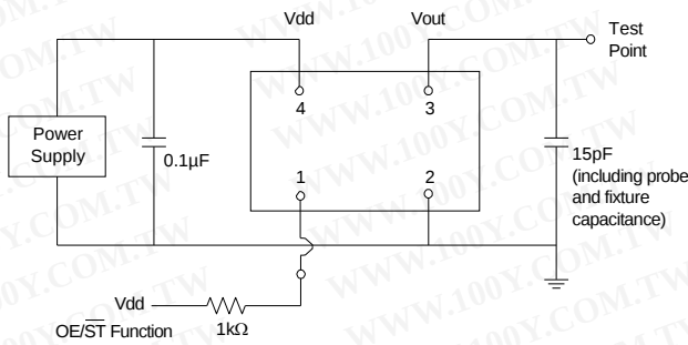
Figure 2. Test Circuit
