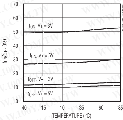
TURN-ON/OFF TIMES vs. TEMPERATURE (MAX4760/MAX4761)
