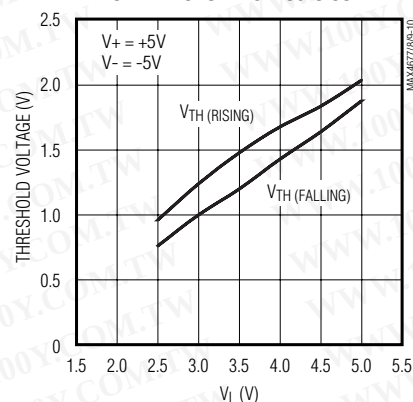
INPUT THRESHOLD vs. LOGIC SUPPLY
