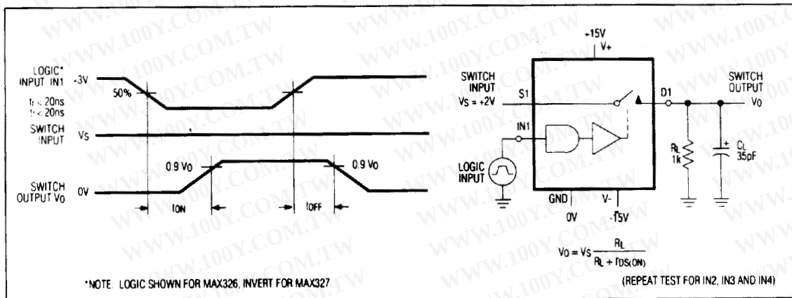
Figure 1. Switching-Time Test Circuit. Switch-output waveform shown for VS = constant with logic-input waveform as shown. Note: VS may be positive or negative as per switching-time test circuit. VO is the steady-state output with switch on. Feedthrough via gate capacitance may result in spikes at leading and trailing edge of output waveform.
