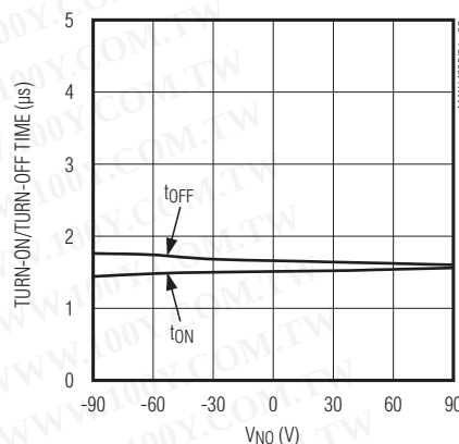
TURN-ON/TURN-OFF TIME vs. ANALOG SIGNAL VOLTAGE
