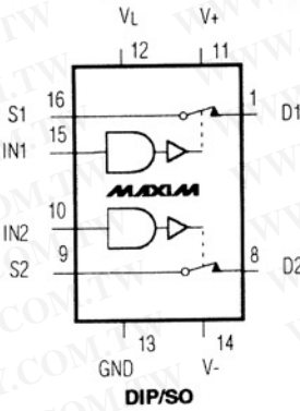
IH5041 Dual SPST
