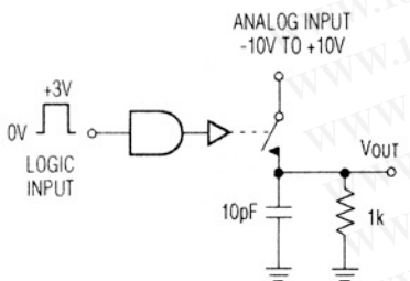
Figure 1. Switching Time
