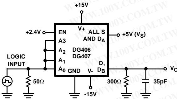
FIGURE 3A. TEST CIRCUIT
