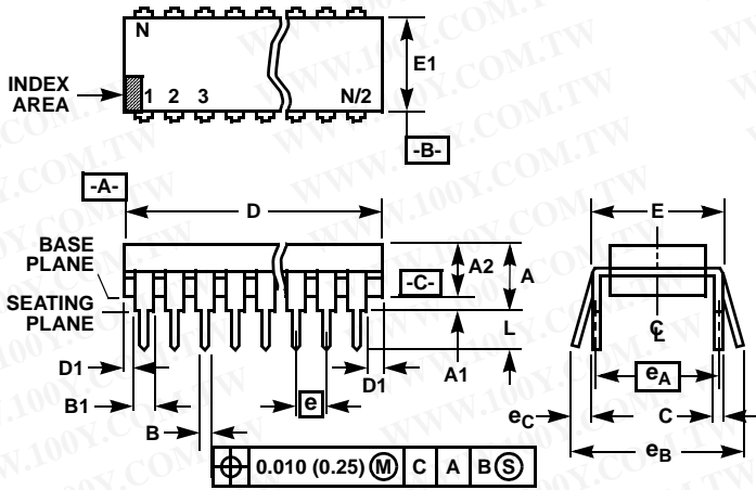
E28.6 (JEDEC MS-011-AB ISSUE B) 28 LEAD DUAL-IN-LINE PLASTIC PACKAGE
