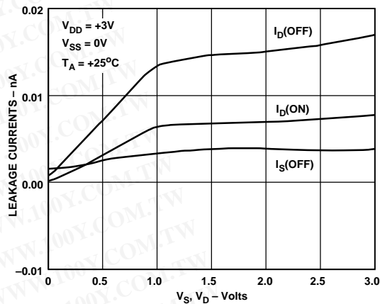
Figure 10. Leakage Currents as a Function of V_D ( V_S )
