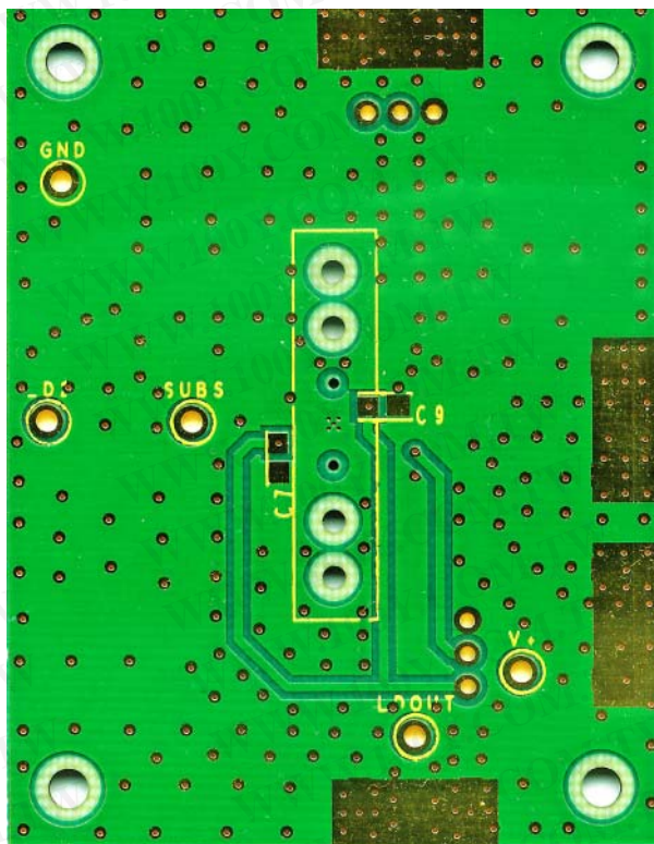
Figure 19. Evaluation Board—Back
