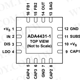
Figure 4. Pin Configuration
