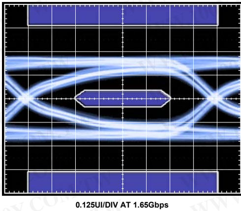
Figure 5. RX Eye Diagram at TP2 (Cable = 2 meters, 30 AWG)
