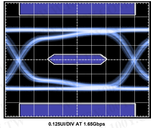
Figure 7. RX Eye Diagram at TP3, EQ = 6 dB (Cable = 2 meters, 30 AWG)
