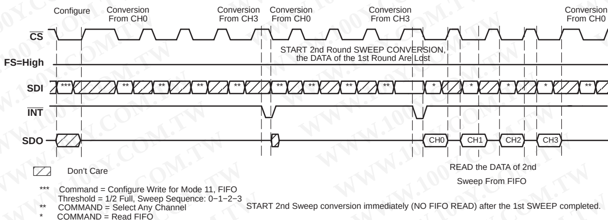
Figure 18. Mode 11, \overline{\text{CS}} Initiates Operations
