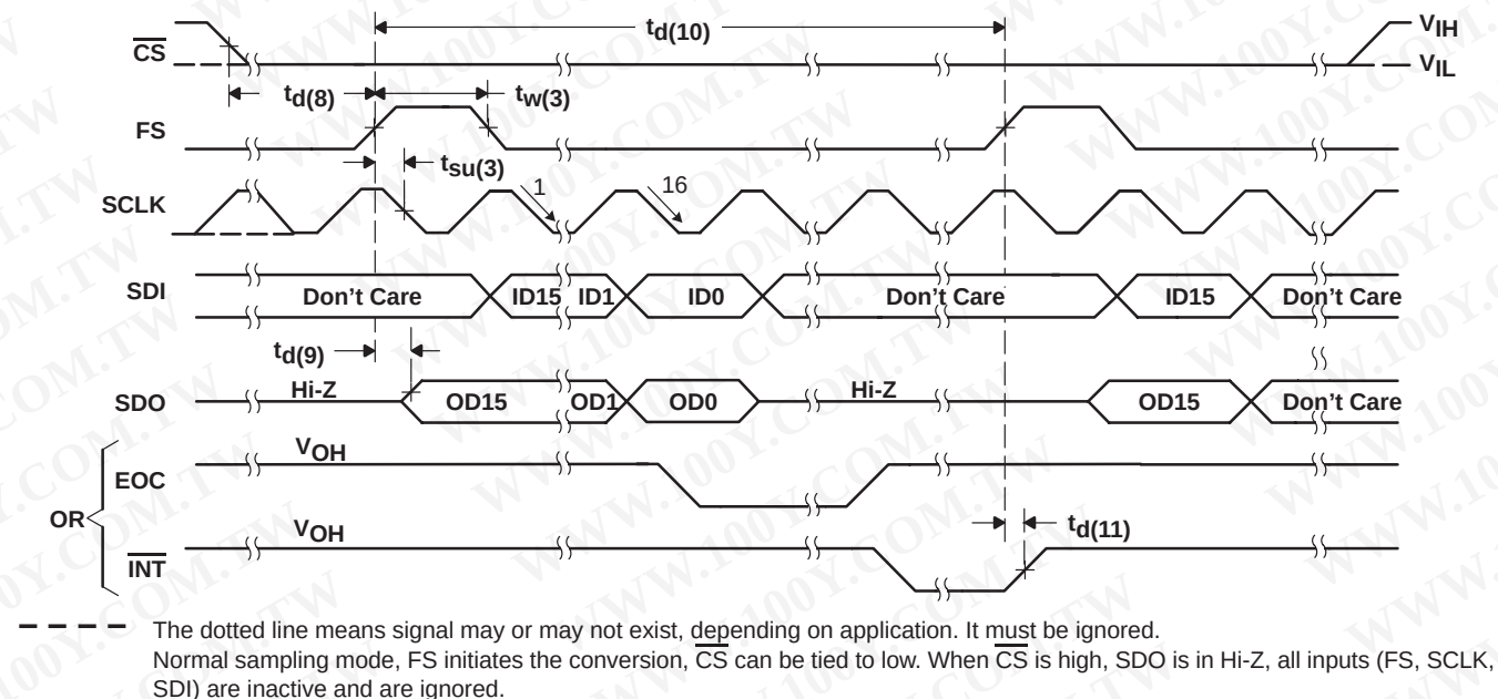
Figure 3. Critical Timing for FS Trigger
