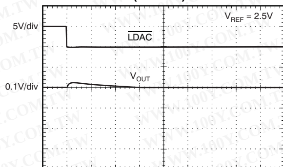
MAJOR-CARRY GLITCH (FALLING)
