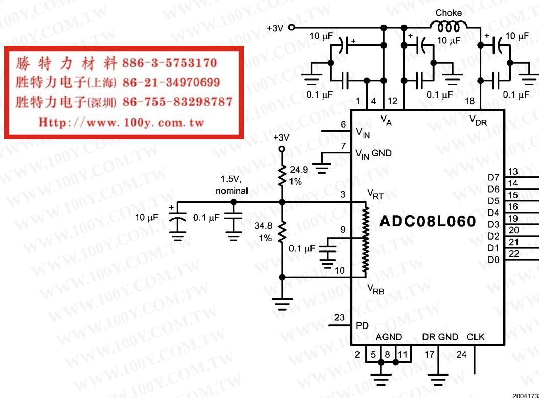
FIGURE 2. Simple, low component count reference biasing. Because of the ladder and external resistor tolerances, the reference voltage of this circuit can vary too much for some applications.
