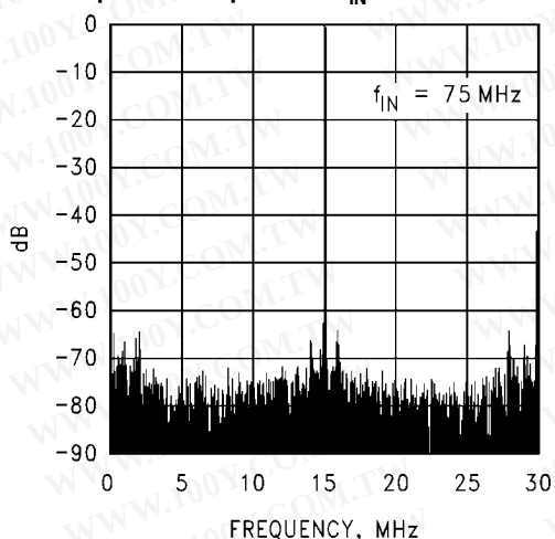
Spectral Response @ f_{IN} = 75 \text{ MHz}
