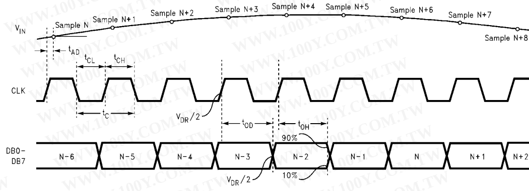
FIGURE 1. ADC08L060 Timing Diagram
