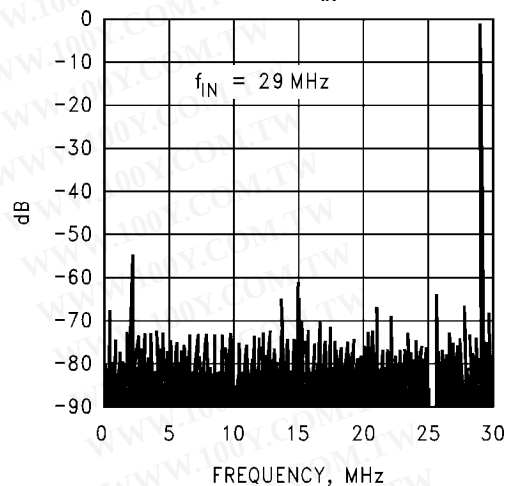
Spectral Response @ f_{IN} = 29 \text{ MHz}
