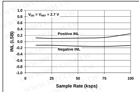
FIGURE 2-4: Integral Nonlinearity (INL) vs. Sample Rate ( V_{DD} = V_{REF} = 2.7V ).
