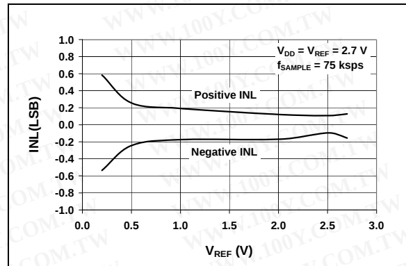
FIGURE 2-5: Integral Nonlinearity (INL) vs. V_{REF} ( V_{DD} = V_{REF} = 2.7V ).
