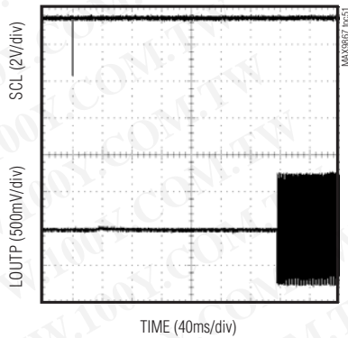
SHUTDOWN TO DAC FULL OPERATION (CLICKLESS SINGLE-ENDED MODE)
