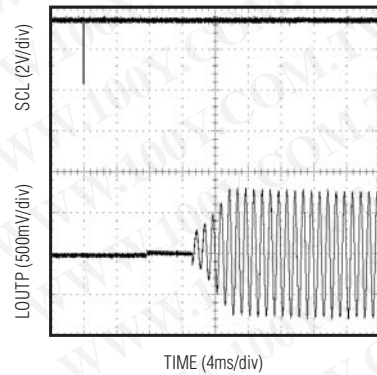
SHUTDOWN TO DAC FULL OPERATION (FAST TURN-ON SINGLE-ENDED MODE)
