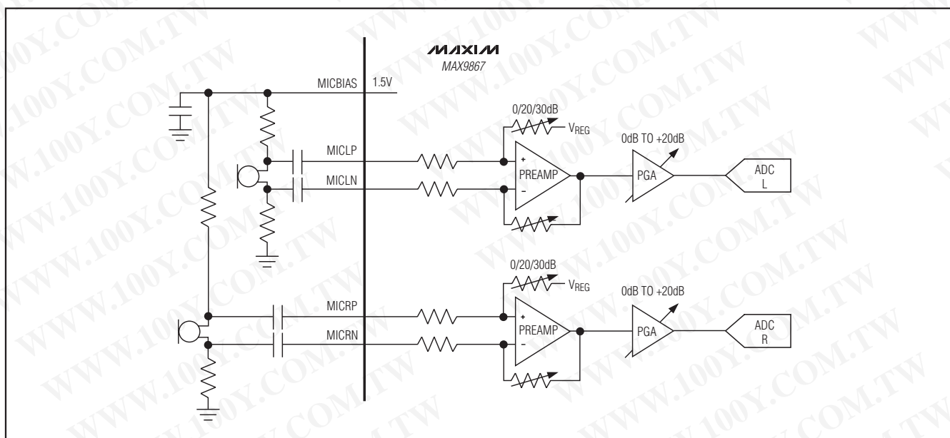
Figure 5. Microphone Input Signal Path
