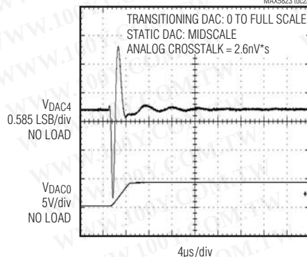
CHANNEL-TO-CHANNEL FEEDTHROUGH ( V_{DD} = 5\text{V} , V_{REF} = 4.096\text{V} , T_A = +25^\circ\text{C} , NO LOAD)
