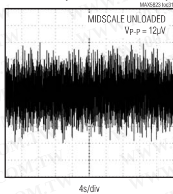
0.1Hz TO 10Hz OUTPUT NOISE, EXTERNAL REFERENCE ( V_{DD} = 5\text{V} , V_{REF} = 4.5\text{V} )
