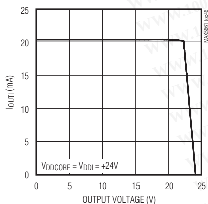
OUTI OUTPUT CURRENT vs. OUTPUT VOLTAGE
