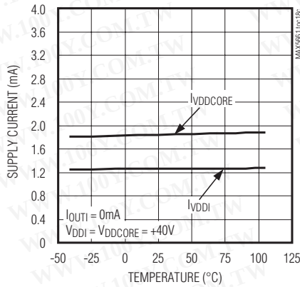
SUPPLY CURRENT vs. TEMPERATURE (0 TO 20mA CURRENT OUTPUT)
