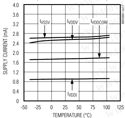
SUPPLY CURRENT vs. TEMPERATURE (BIPOLAR VOLTAGE OUTPUT)
