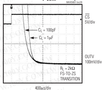
UNIPOLAR VOLTAGE-OUTPUT SETTLING TIME ( C_{COMP} = 3.3nF )
