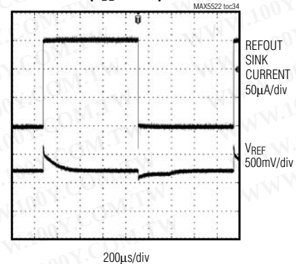
REFERENCE LOAD TRANSIENT ( V_{DD} = 1.8V )
