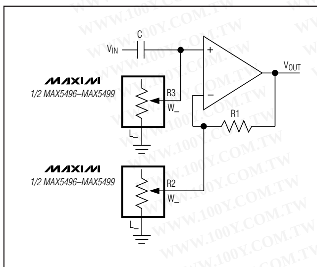
Figure 14. Programmable Filter
