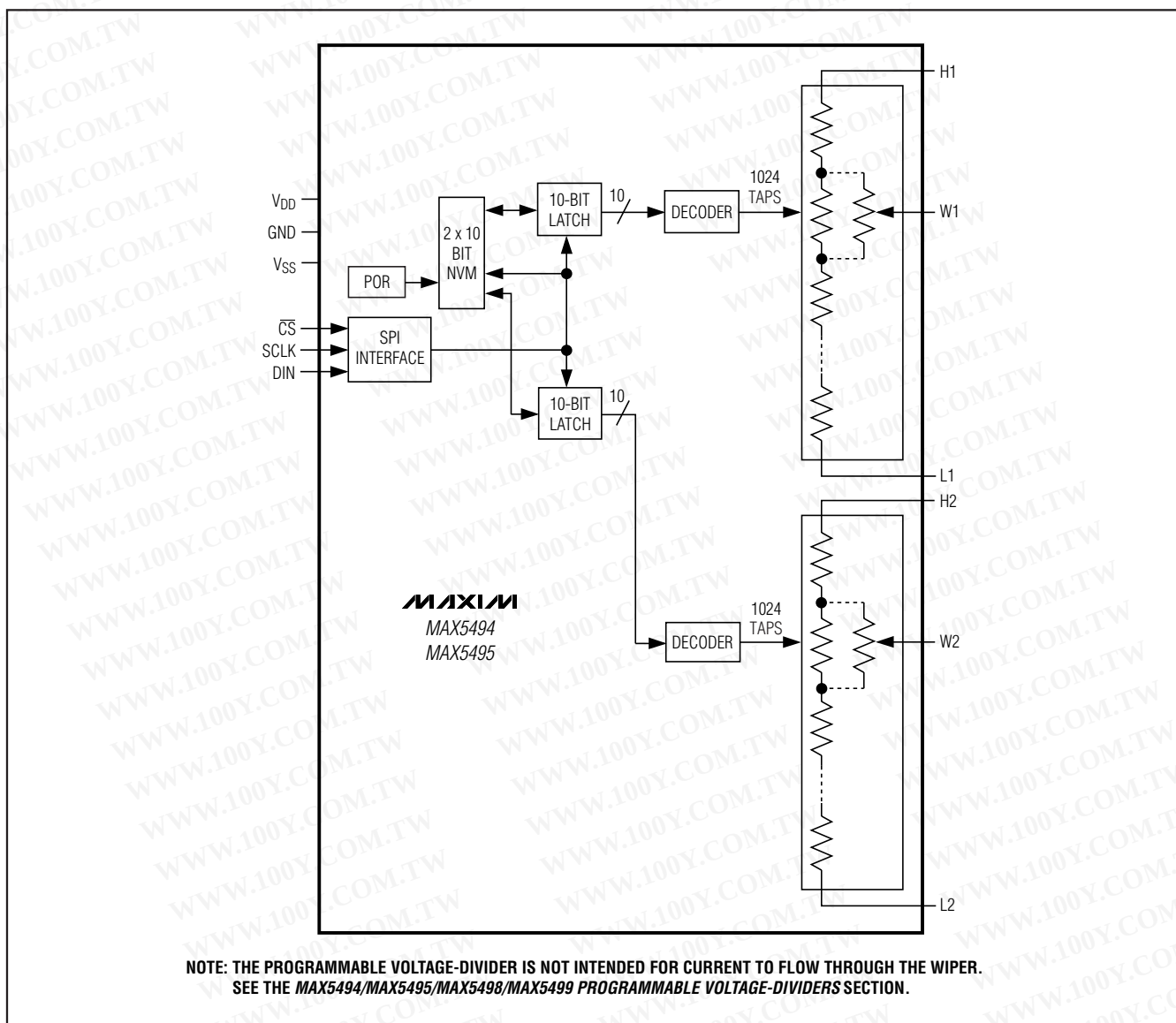
Figure 1. MAX5494/MAX5495 Functional Diagram
