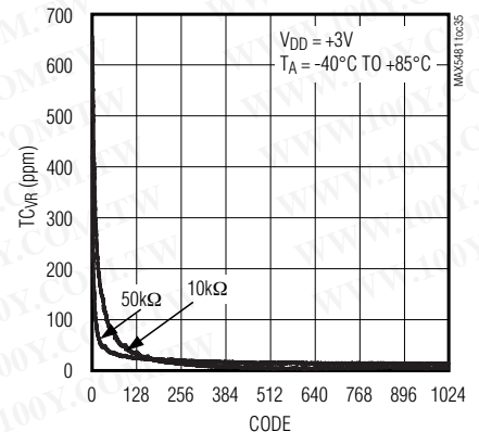
VARIABLE-RESISTOR TEMPERATURE COEFFICIENT vs. CODE
