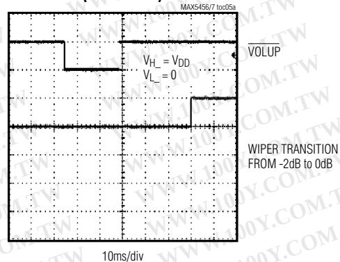
WIPER SWITCHING TRANSIENT (TIMING OUT)
