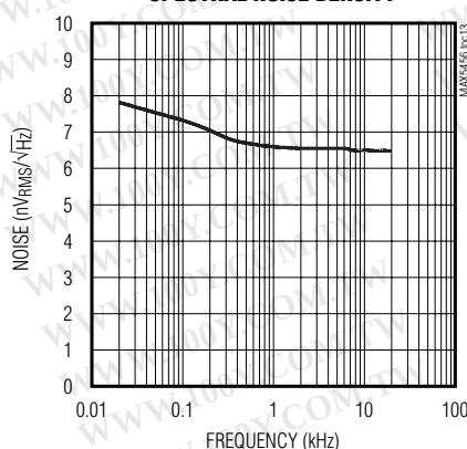
SPECTRAL NOISE DENSITY
