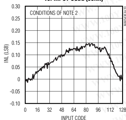
VARIABLE-RESISTOR INL vs. INPUT CODE (50k \Omega )
