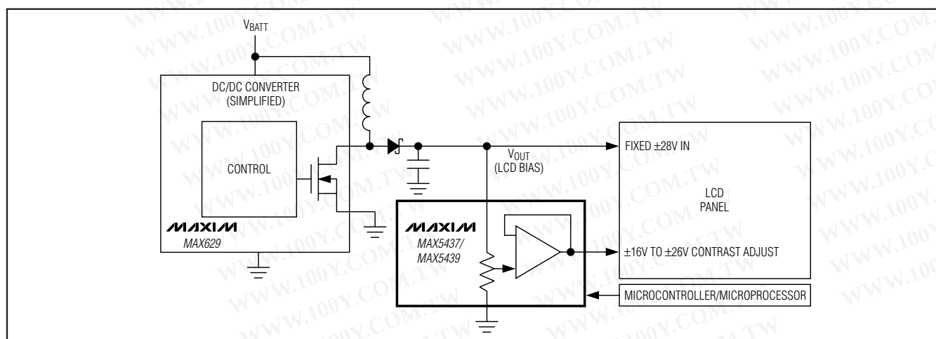
Figure 5b. Simplified LCD Contrast Control Circuit with Buffer
