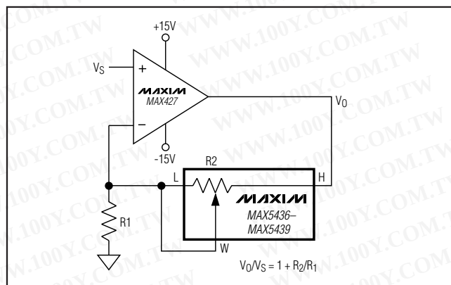
Figure 4. Noninverting Amplifier
