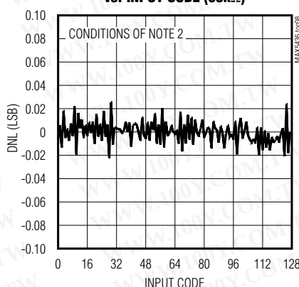
VARIABLE-RESISTOR DNL vs. INPUT CODE (50k \Omega )
