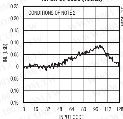
VARIABLE-RESISTOR INL vs. INPUT CODE (100k \Omega )
