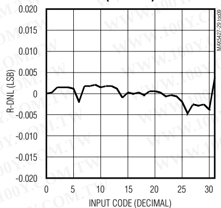
R-DNL ERROR vs. INPUT CODE (MAX5428)
