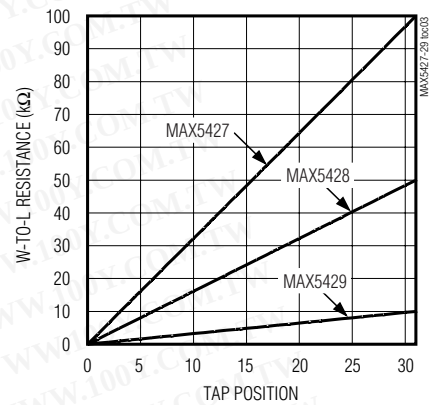
W-TO-L RESISTANCE vs. TAP POSITION
