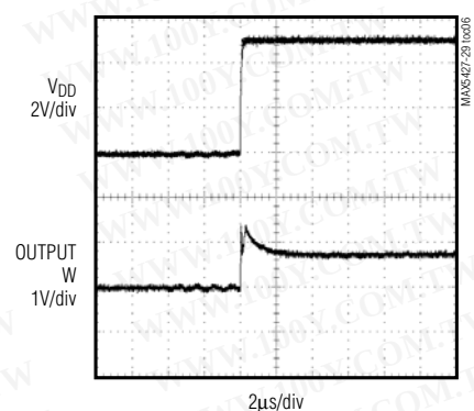
WIPER TRANSIENT AT POWER-ON
