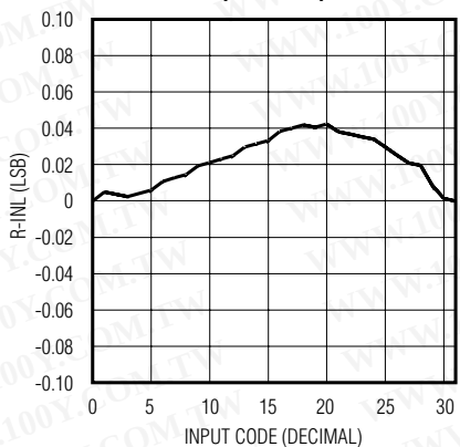
R-INL ERROR vs. INPUT CODE (MAX5427)
