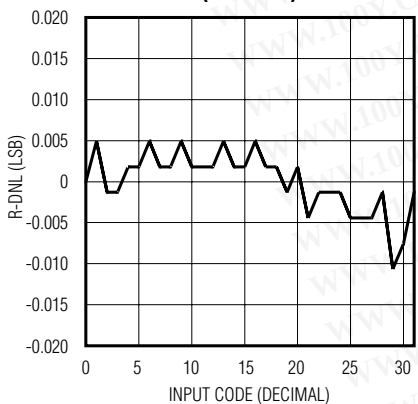
R-DNL ERROR vs. INPUT CODE (MAX5427)
