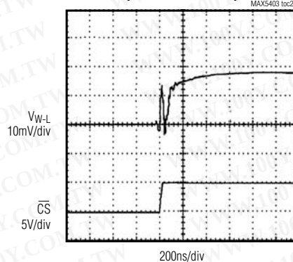
TAP-TO-TAP SWITCHING TRANSIENT (CODE 127 TO 128)
