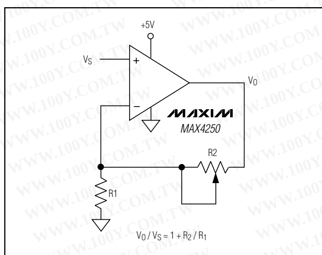
Figure 6. Noninverting Amplifier
