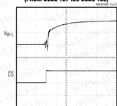
TAP-to-TAP SWITCHING TRANSIENT (FROM CODE 127 to CODE 128)
